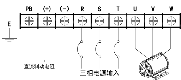
d) 37KW-45KW 变频器主回路端子排配线图
