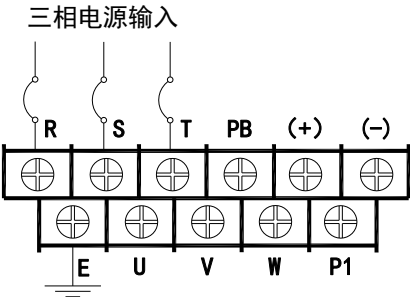
i) 280kW-450kW 变频器主回路端子排配线图
